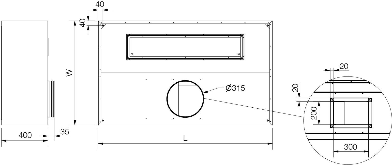
Circular connection details
