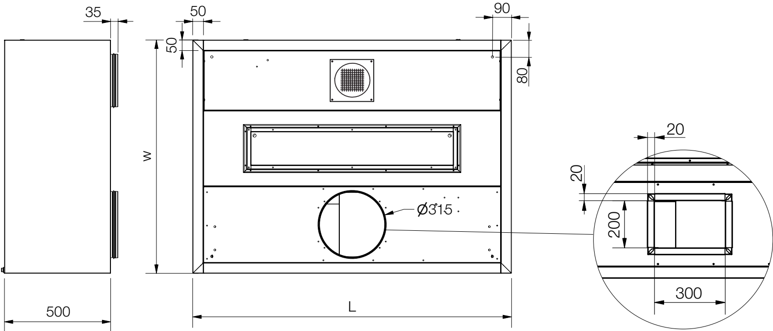
Circular connection details
