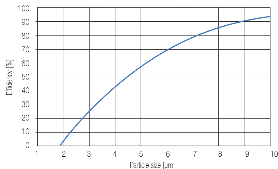
Diagram of particle separation efficiency per particle size. Tests are conducted at 130Pa filter pressure drop and 1500 [ \text{m}^3/\text{h} \cdot \text{m} ] of exhaust airflow.
