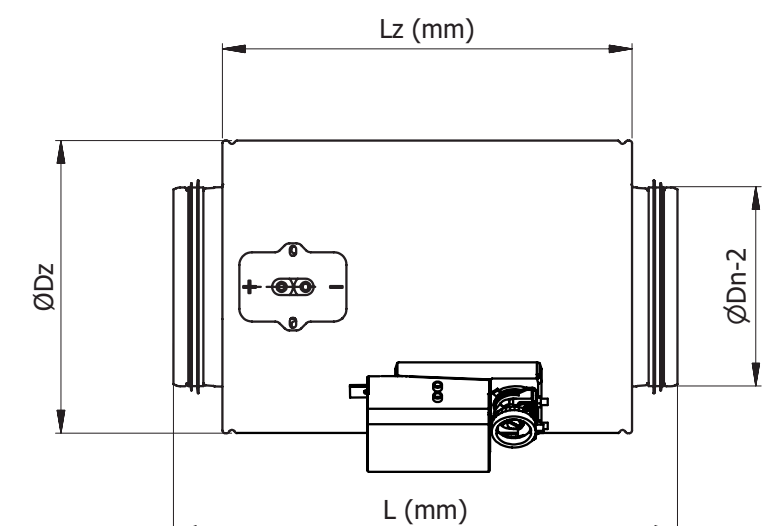
RVP-C-Z (Insulated casing)
