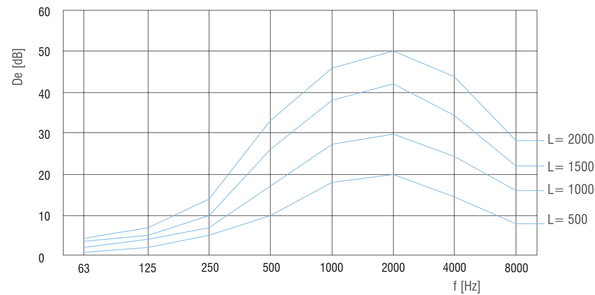
Attenuation diagram, type PZ 100/100
