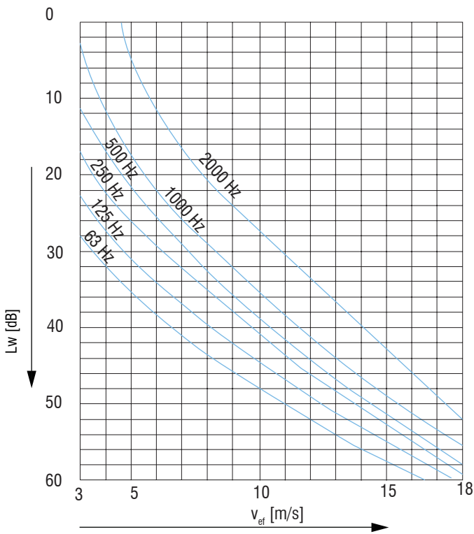
Airflow regenerated noise diagram for d/s = 100/100 (based on outlet size B \times H = A_{tot} = 1\text{m}^2 )
