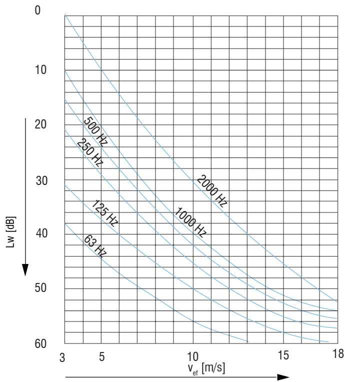
Airflow regenerated noise diagram for d/s = 100/50 (based on outlet size B \times H = A_{tot} = 1\text{m}^2 )
