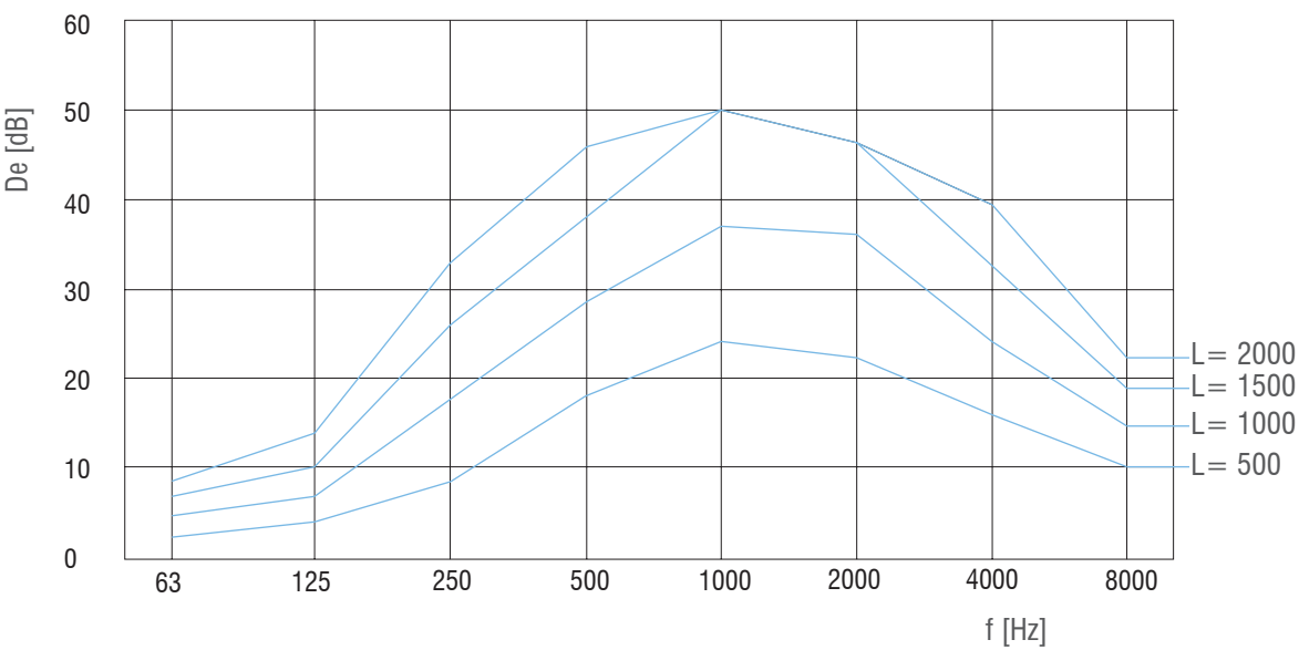
Attenuation diagram, type PZ 200/100
