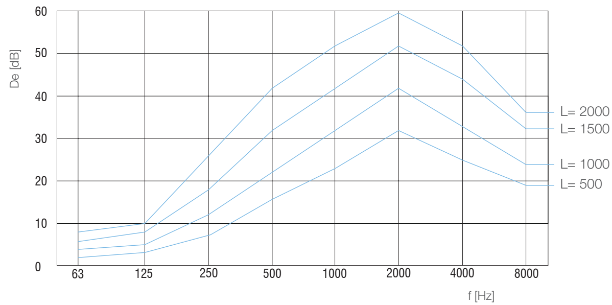
Attenuation diagram, type PZ 100/50
