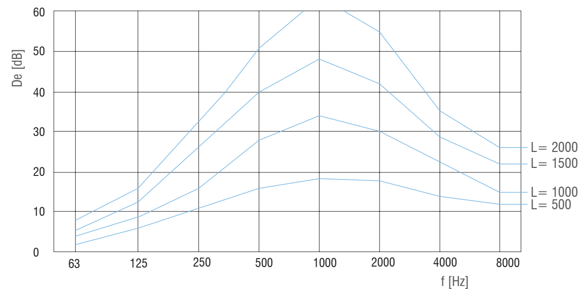
Attenuation diagram, type PZ-R 100/50
