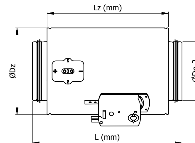
RVP-C-Z (Insulated casing)
