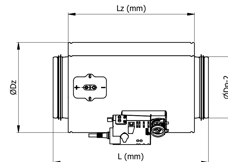
RVP-C-Z (Insulated casing)
