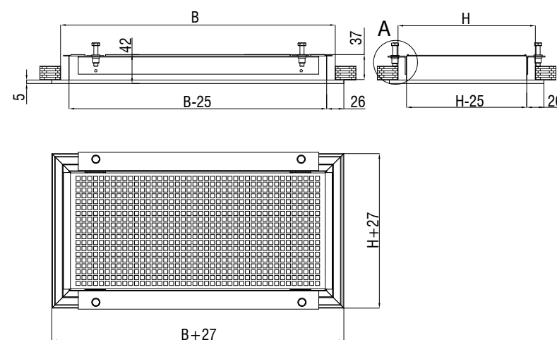
Detail A
